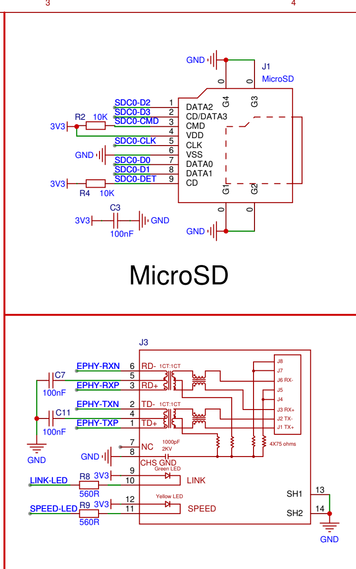
Ethernet (10/100M)
