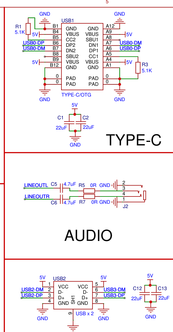
USB X 2
