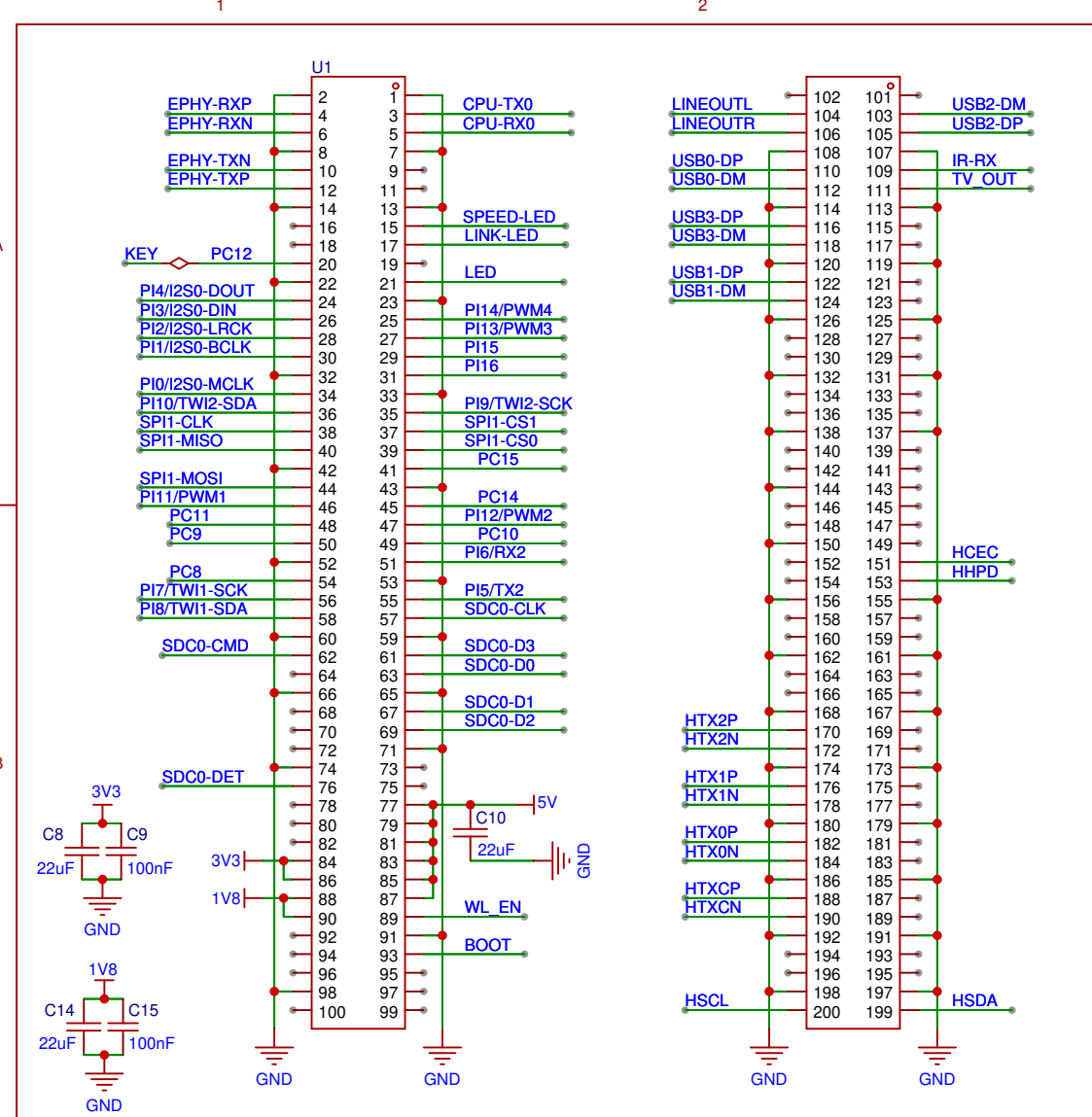
WalnutPi Compute Module Connector
